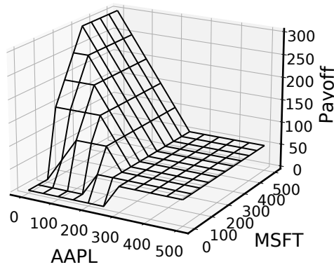
Fig. 2. Payoff of combinatorial options matched in Example 3 as a function of S_{\text{AAPL}} and S_{\text{MSFT}} . The example demonstrates the case of L = 0 .
