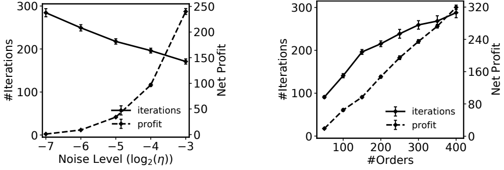
(a) Vary noise \eta added to order prices in markets with U = 4 and n_{\text{orders}} = 150 .
